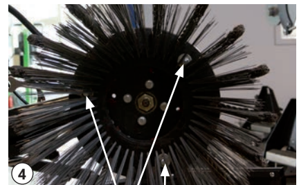
Three nuts
